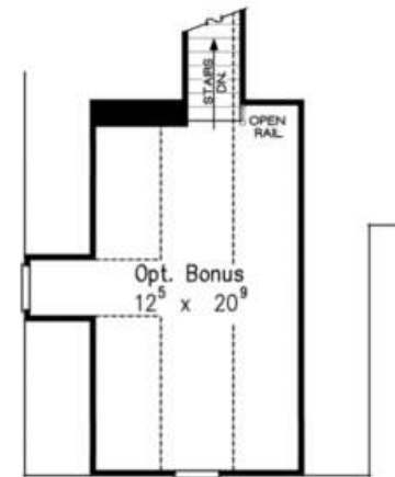
OPTIONAL SECOND FLOOR PLAN
